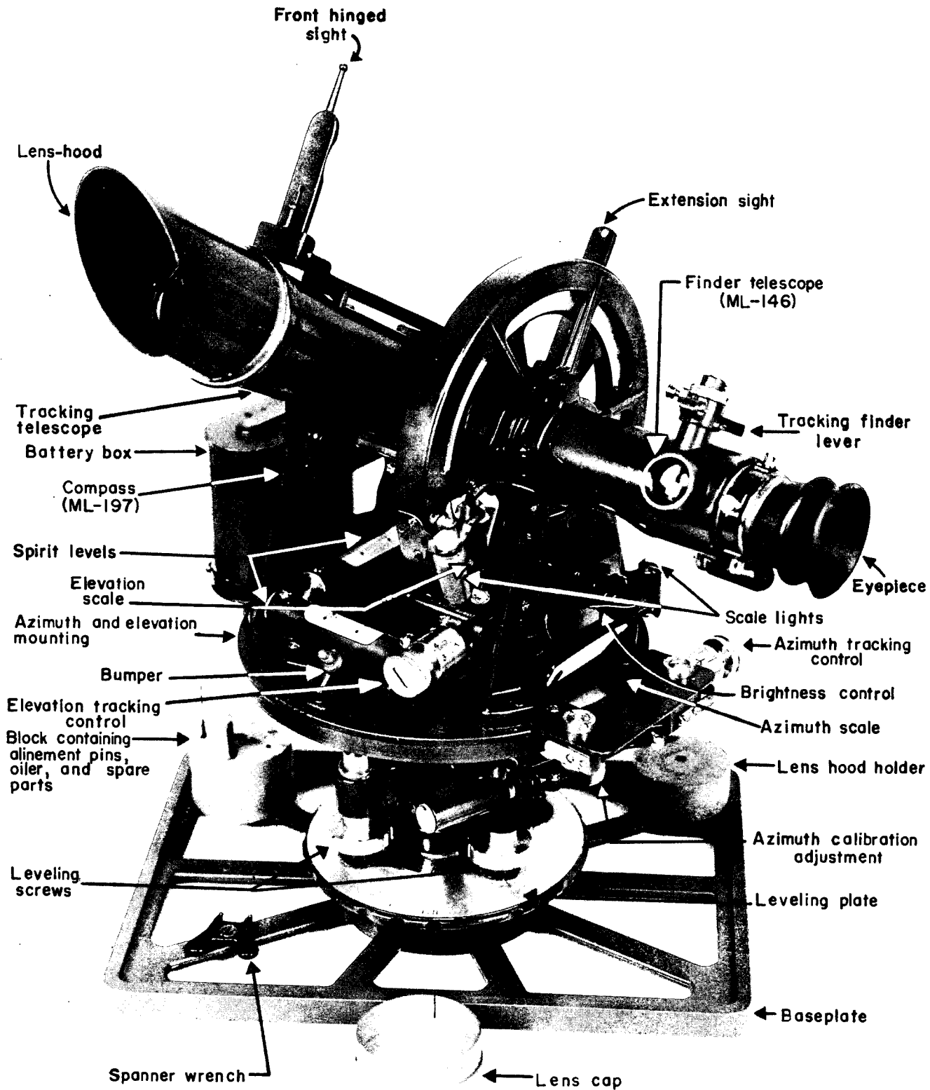
Figure 29. Theodolite ML-474/GM.
