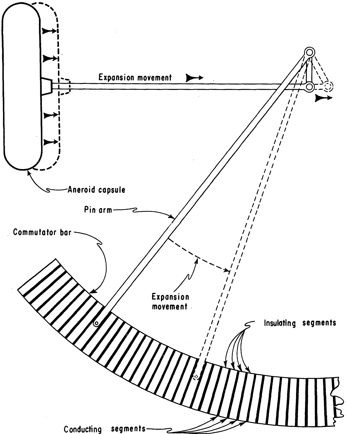
Figure 46. Action of baroswitch.
