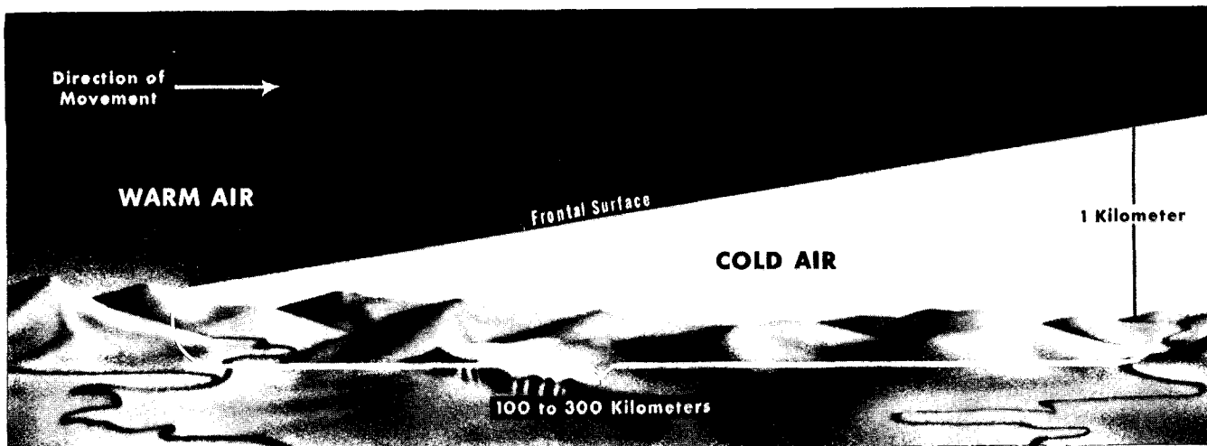
Figure 11. Warm front.
