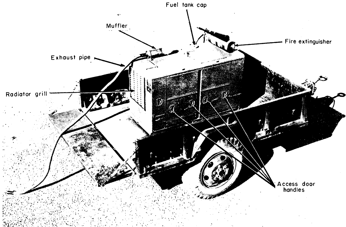
Figure 58. Power unit, 10-kw.
