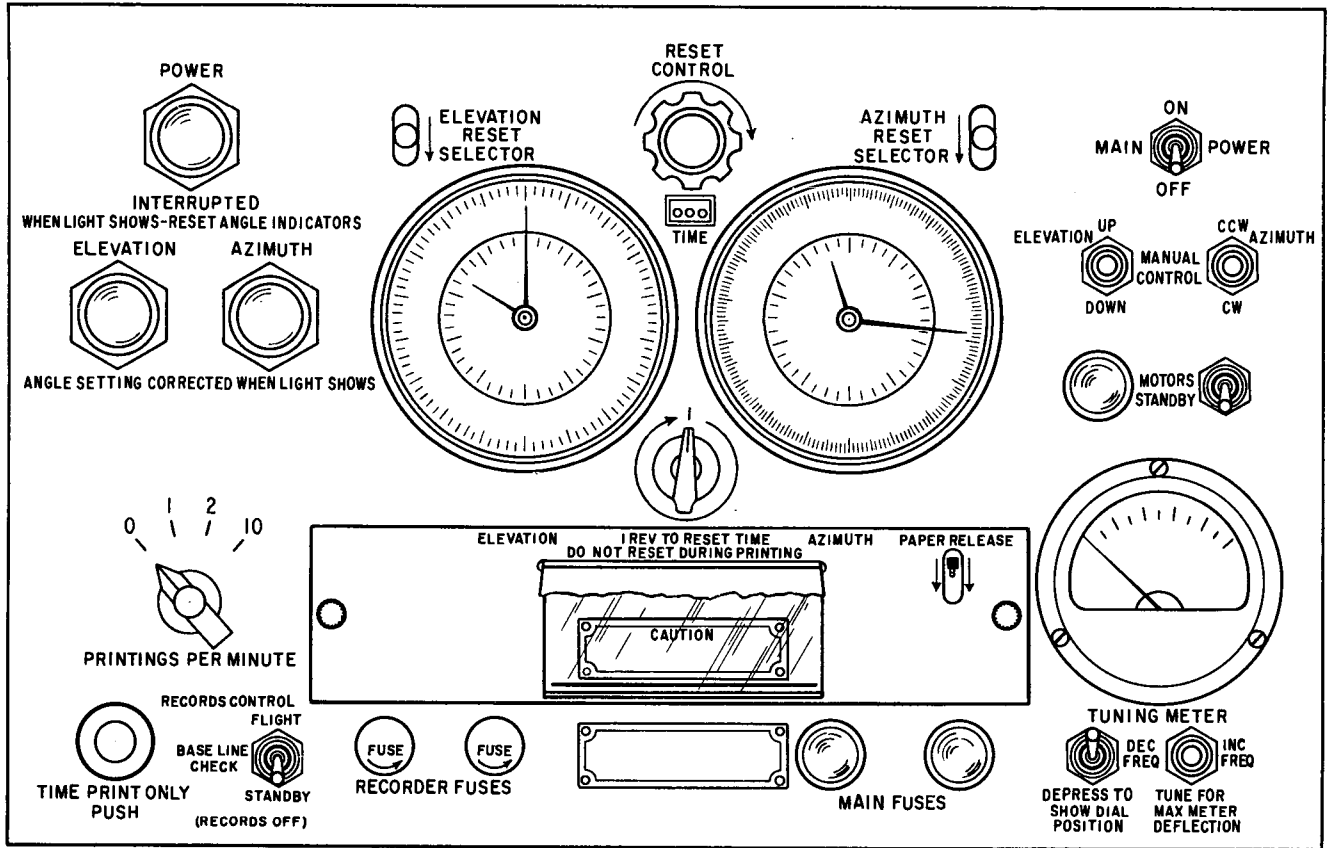
Figure 51. Control-recorder.
