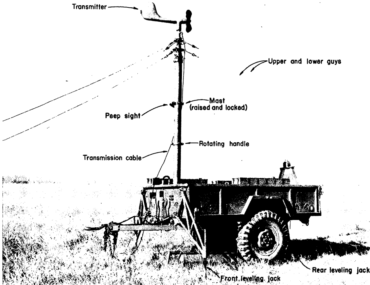
Figure 189. Wind measuring set AN/MMQ-1( ).
