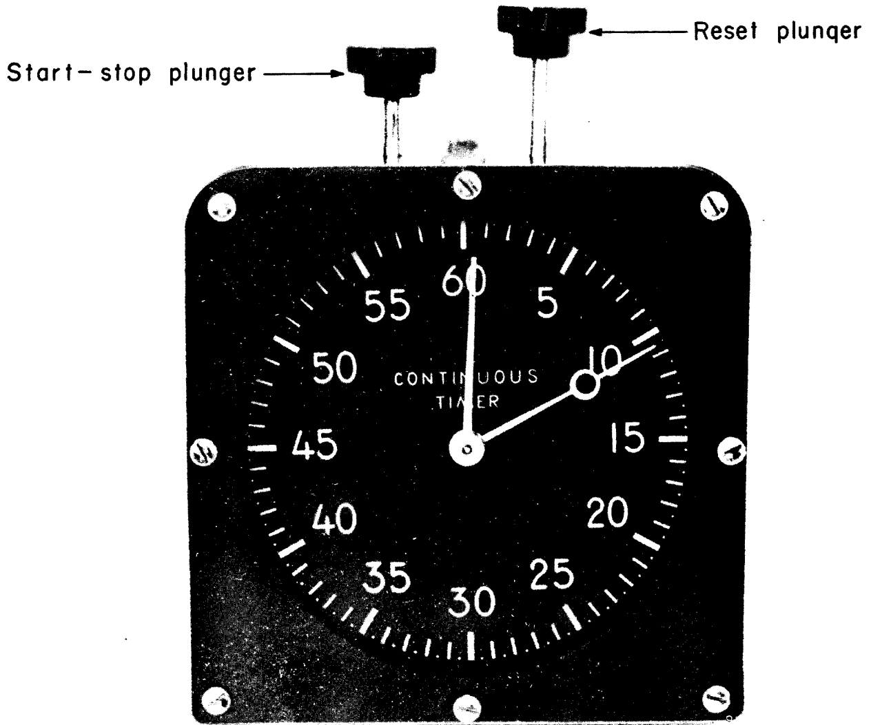
Figure 30. Timer FM-19.
