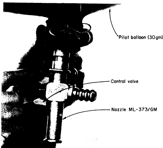
Figure 39. Nozzle ML-373/GM.
