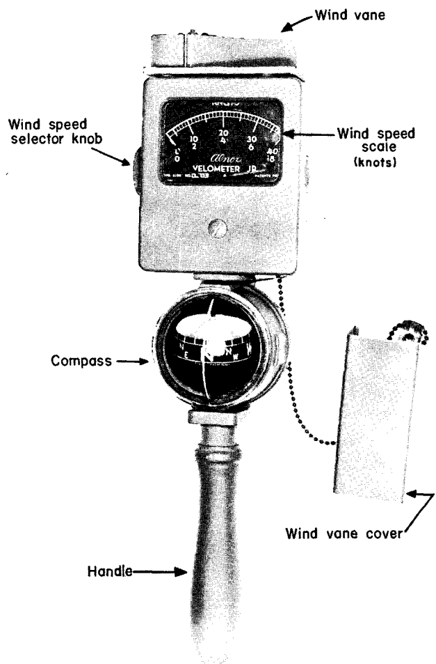
Figure 25. Anemometer ML-433/PM.
