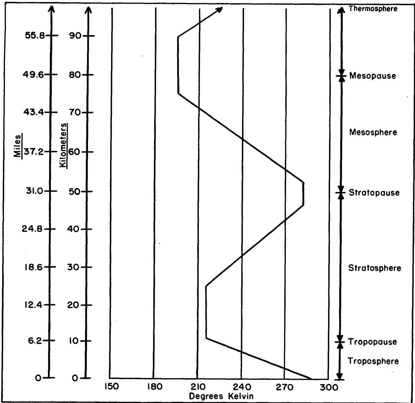
This chart is based on NATO STANAG 4044 (1958). ICAO up to 20 kilometers; U.S. Ext. to ICAO above 20 kilometers.
