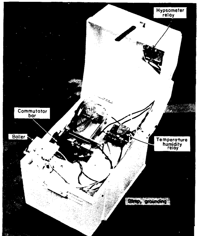
Figure 47. Radiosonde set AN/AMT-12 (hypsometer).
