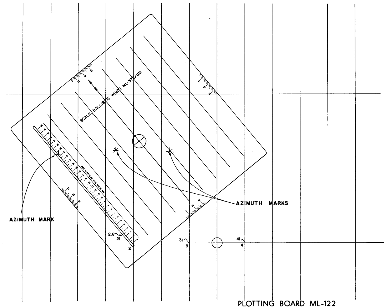
Figure 105. Plotting ballistic wind speeds.
