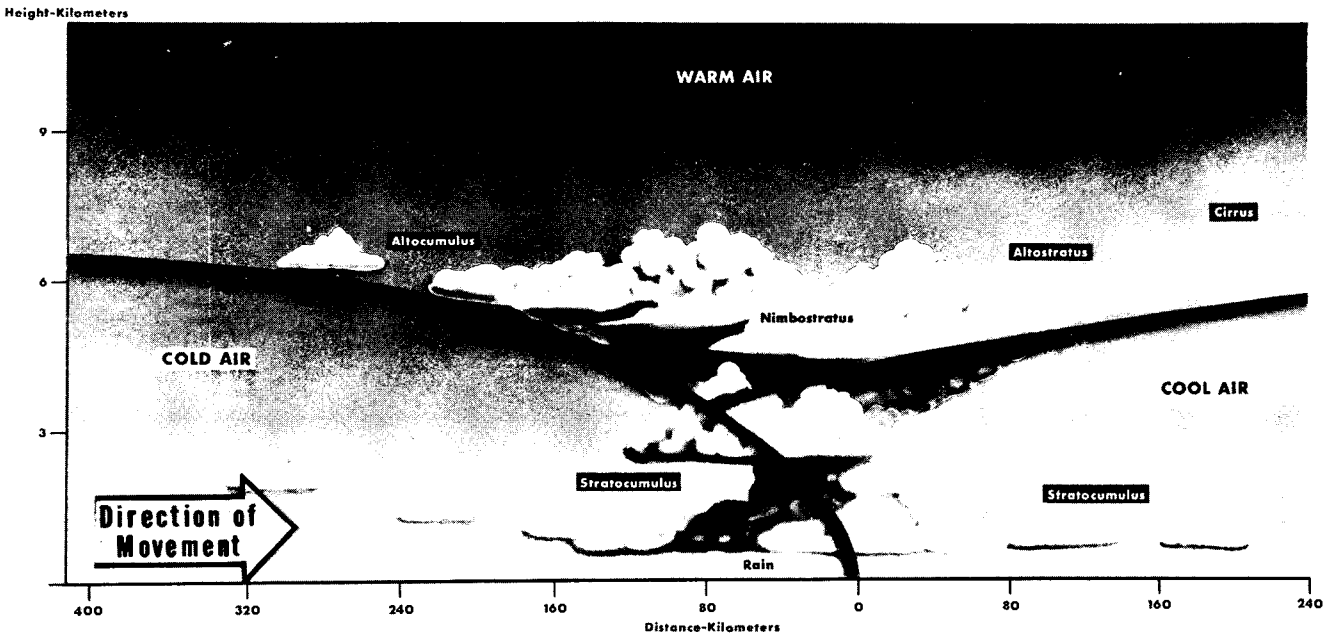
Figure 14. Cold front occlusion.
