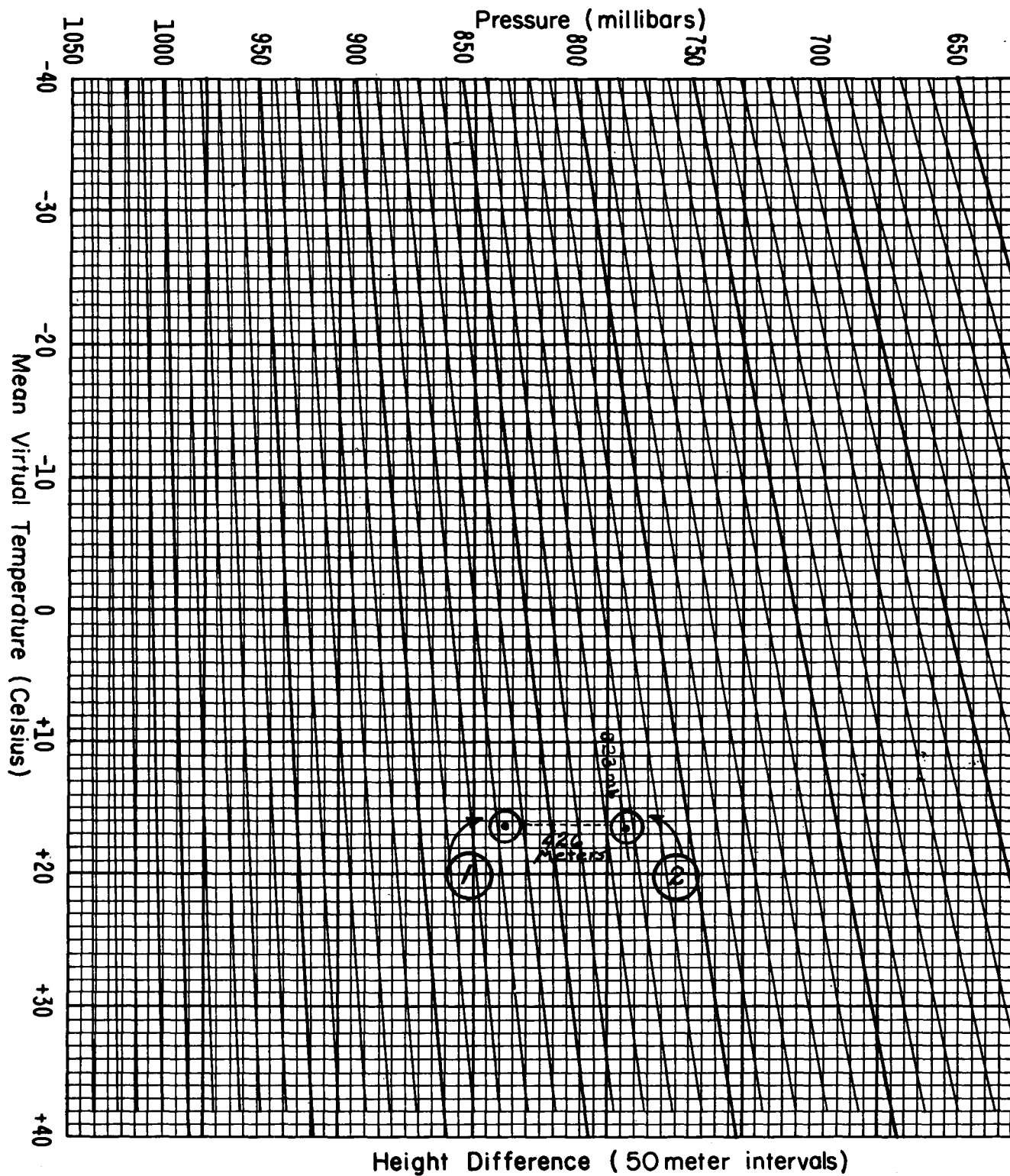
Figure 144. Pressure-height chart.
