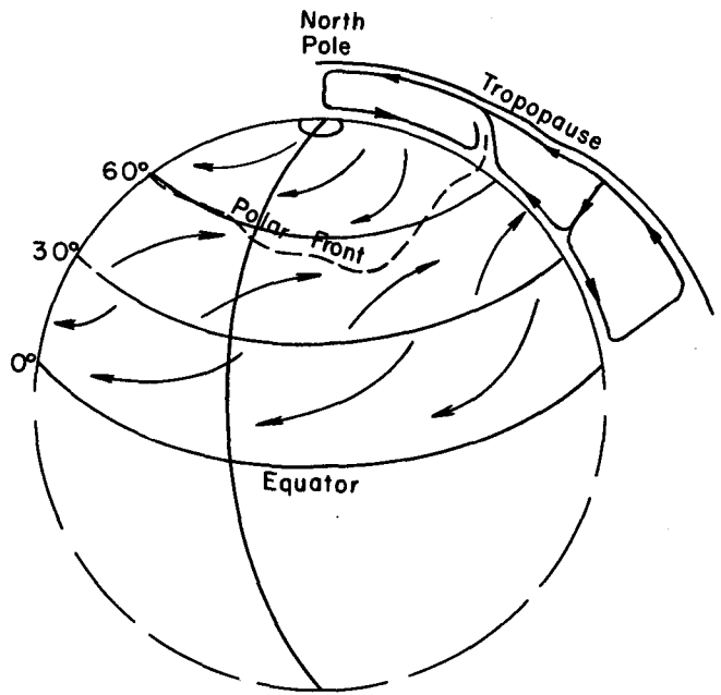
Figure 5. General circulation.
