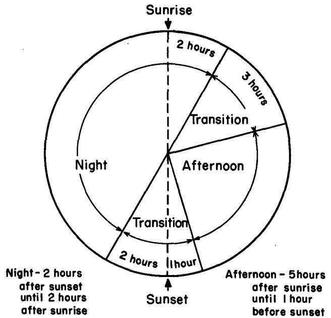
Figure 113. Meteorological day.
