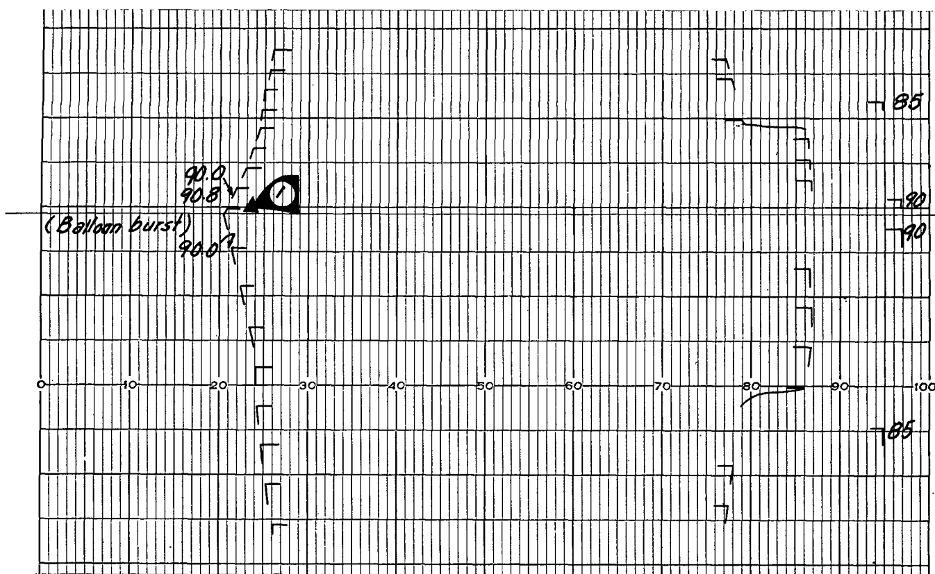
Figure 72. Terminal layer.
