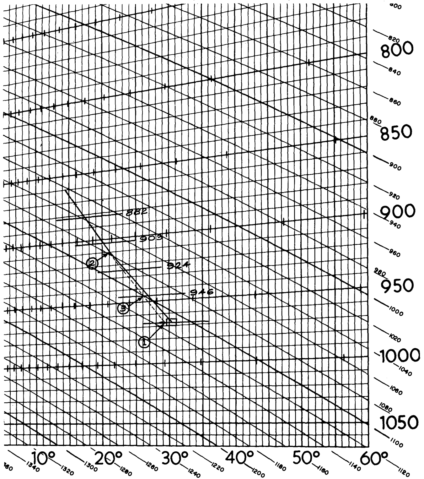
★Figure 125. Sound ranging layers plotted on chart ML-574/UM.
