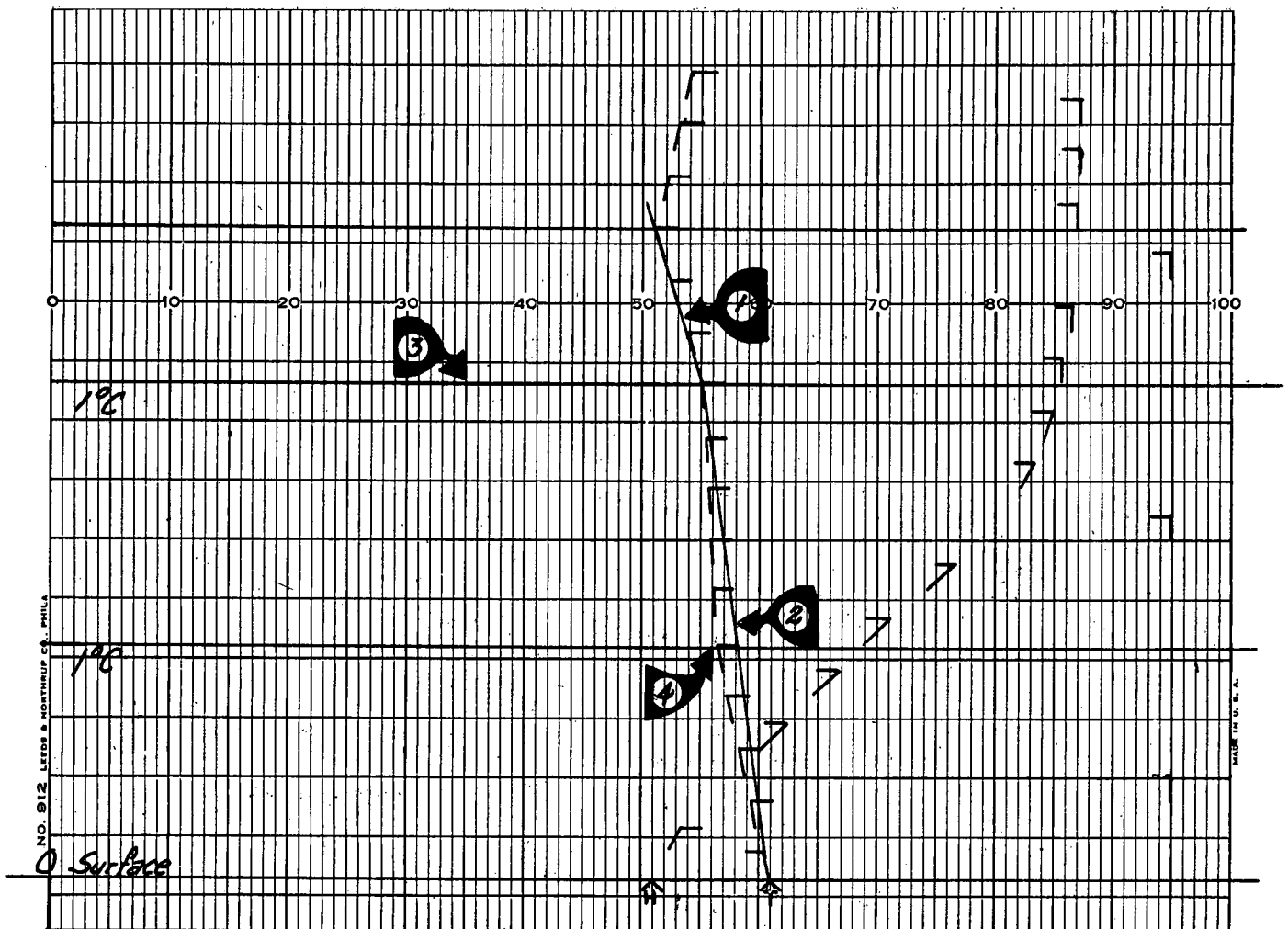
Figure 69. Determination of temperature deviation from line of linearity.
