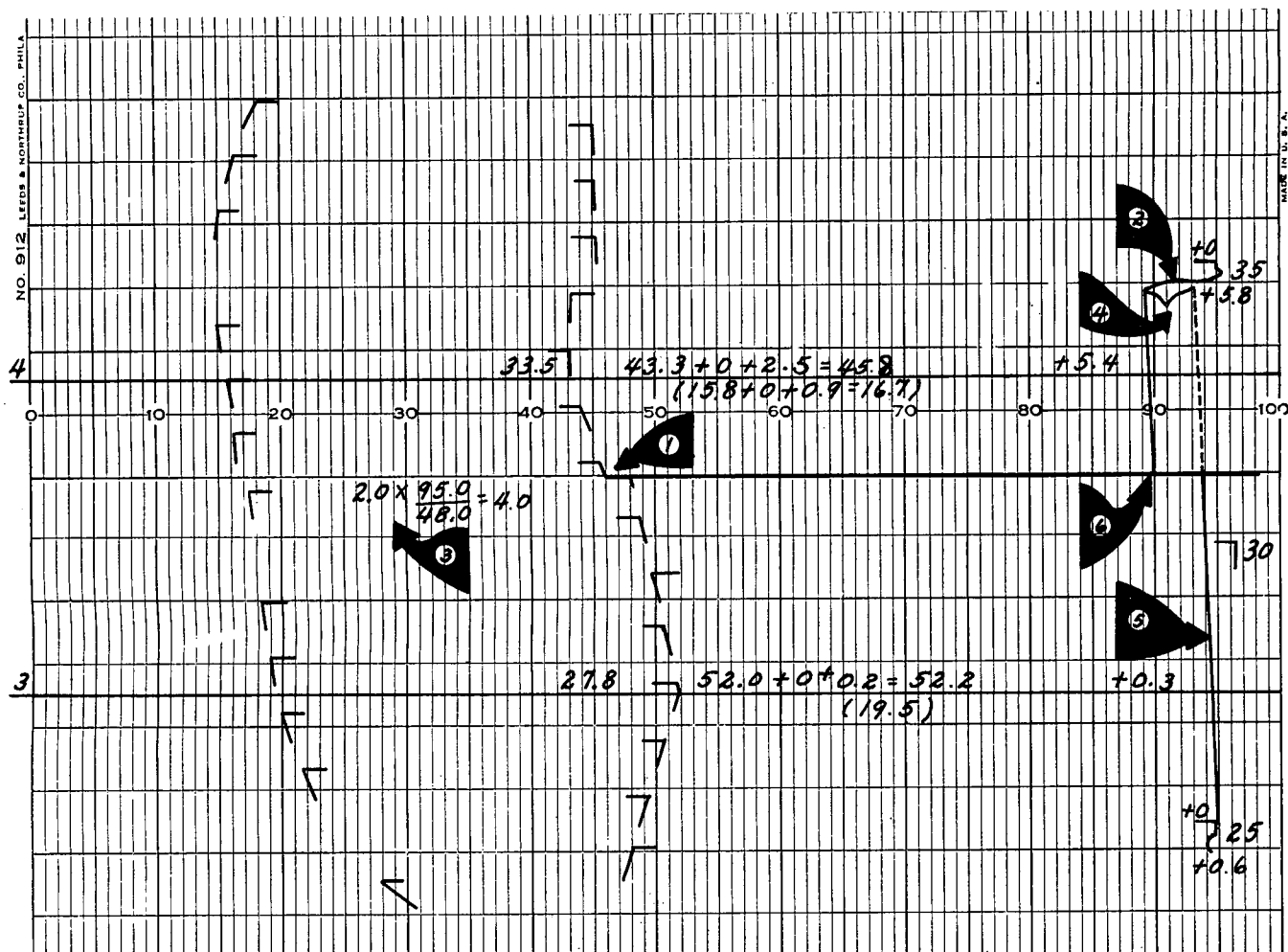
Figure 83. Determining shift or shift plus drift corrections.
