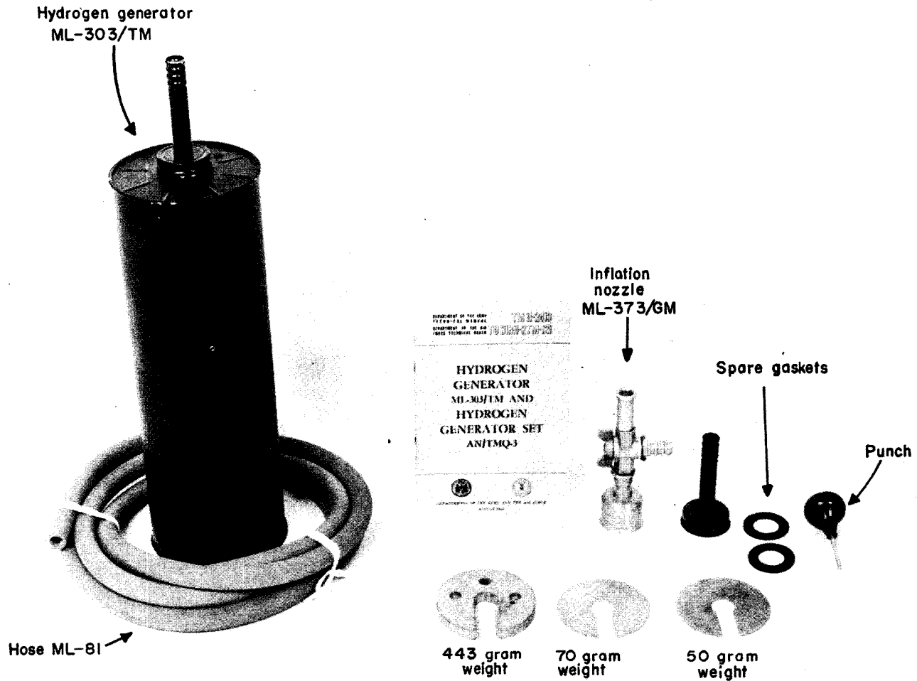
Figure 36. Hydrogen generator ML-303/TM.
